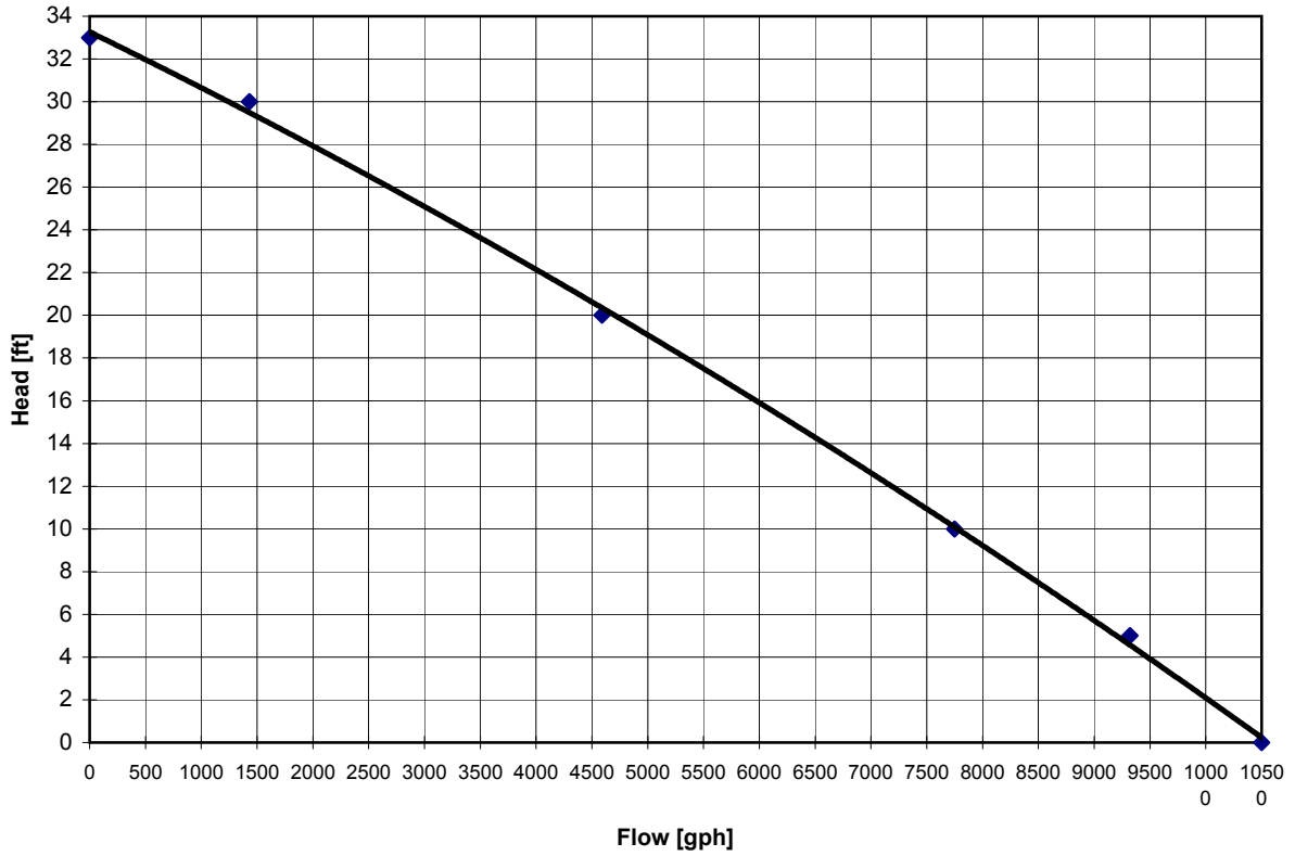
T10000 Pump Curve Torpedo
