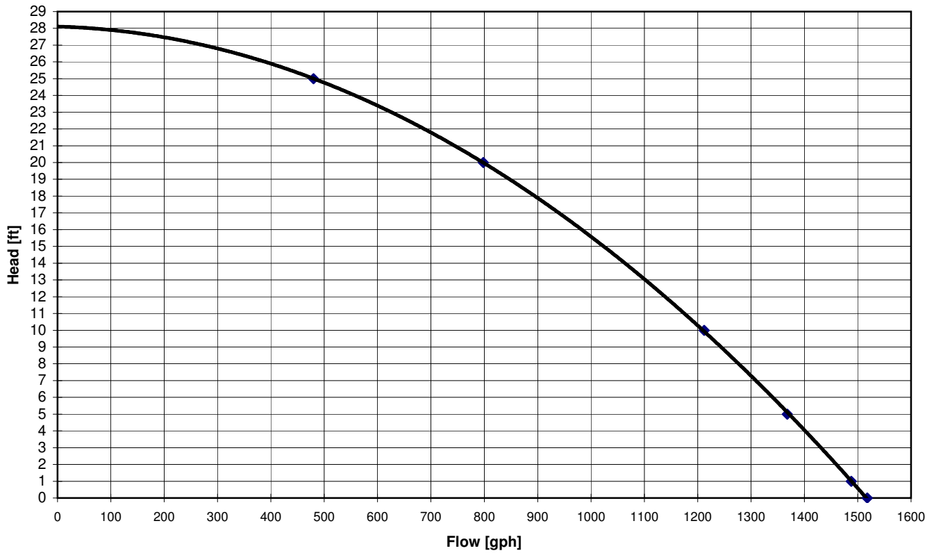
T1500 Pump Curve Torpedo
