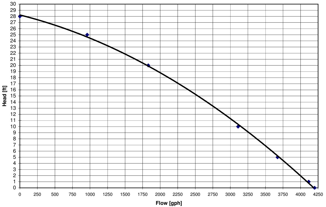
T4000 Pump Curve Torpedo
